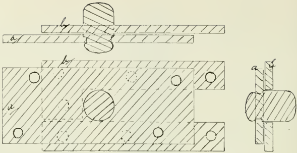
Plan showing mountings for fastening of rib-stalls. a) A piece of metal whose top is riveted on is screwed fast to the rib-stall posts; b) the metal screwed fast to the beam.
