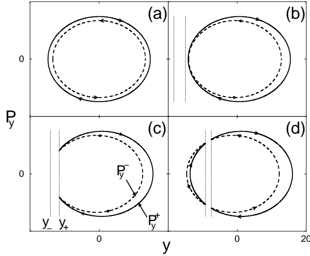
Fig. 1 – Phase space orbits defined by p_y^{\pm,\alpha} given in (4) with |\Delta(y)| = |\Delta| . The solid line is for a particle-like excitation, the dashed line is for a hole-like one. Arrows indicate the direction of the velocity. (a) P_x = 0 . The turning points along the y -axis are given by p_y^{\pm,\alpha} = 0 . (b) P_x \neq 0 and small. The orbits are shifted in opposite directions. The vertical dotted lines indicate the position of the Andreev-like turning points, y_+(P_x) and y_-(P_x) , see equation (6). (c) As P_x increases further the Andreev-like turning point y_+ , for which p_y^{\pm,\alpha} \neq 0 , is reached before the normal turning points given by p_y^{\pm,\alpha} = 0 . MAS takes place (see text). (d) P_x increases even further. Now MAS also occurs at y_- creating a second particle-hole orbit. The two orbits are separated in real space by \delta y = 2|\Delta|/P_x \omega_c .
